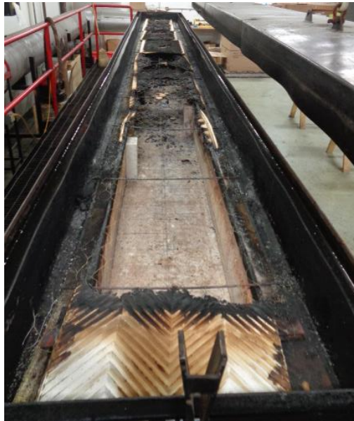
Photo No. 3 Exposed Surface of the Test Specimen (Post-test)
