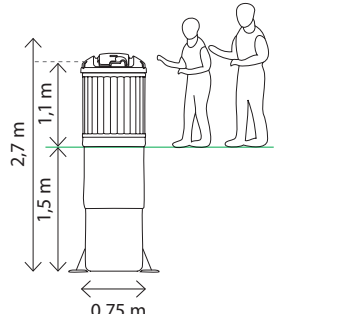
Molok®Classic 800 l
