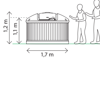
Molok®Classic Light
