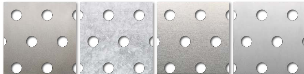
Steel
