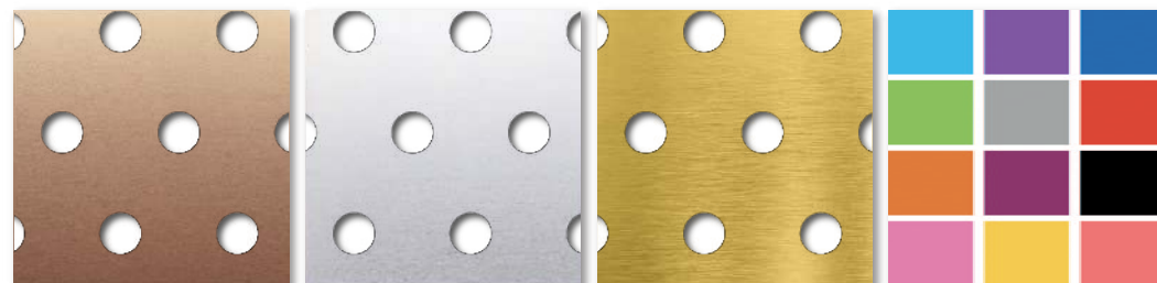
Copper
