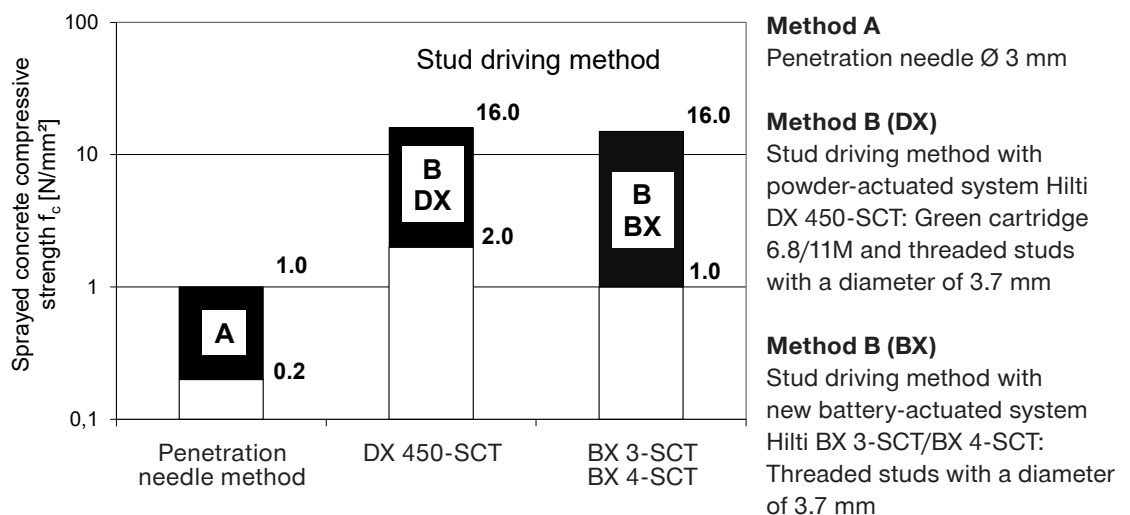
Figure 2: Measurement methods and sprayed concrete strength range
