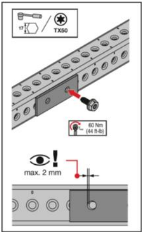
Figure B2: Installation instructions for Hilti MT-TFB OC thread forming bolts
