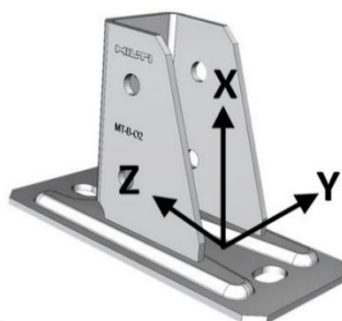
Figure D3: Definition of Hilti MT-B O2, MT-B O2 OC, MT-B O2 FL and MT-B O2 FL OC, baseplate local coordinate system for use with Hilti MT-50 S, MT-50, MT-50 U, MT-50 S OC and MT-50 OC installation channels
