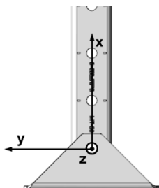
Figure D2: Definition of Hilti MT-AB A set and MT-AB A OC set local coordinate system for use with Hilti MT-50 S, MT-50, MT-50 S OC and MT-50 OC installation channels
