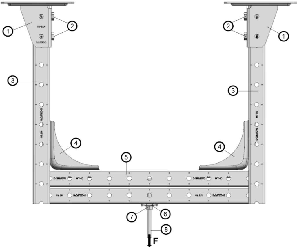
Figure B3: Hilti frame trapeze of MT System with load introduction components, MT-50 and MT-40D, MT-40D V2 or MT-50D channels
