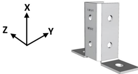
Figure D4: Definition of Hilti MT-B-T, MT-B-T OC, MT-B-T 10, MT-B-T 10 OC, MT-B-T 10 FL, MT-B-T 10 FL OC, MT-B-T FL and MT-B-T FL OC baseplate local coordinate system for use with Hilti MT-50 S, MT-50, MT-50 U, MT-50 S OC and MT-50 OC installation channels
