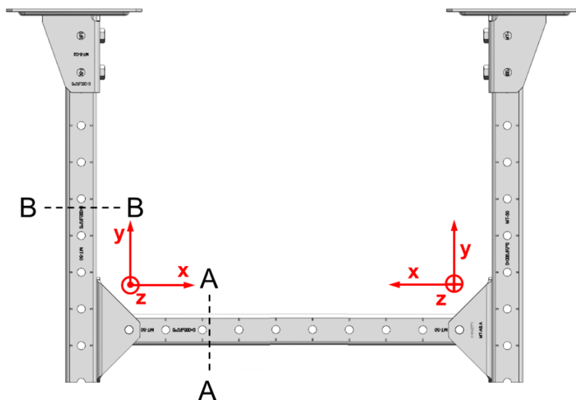
Figure D6: Definition of Hilti MT-AB A set and MT-AB A OC set local coordinate system and viewpoints for use with Hilti MT-50 S, MT-50, MT-50 S OC and MT-50 OC installation channels
