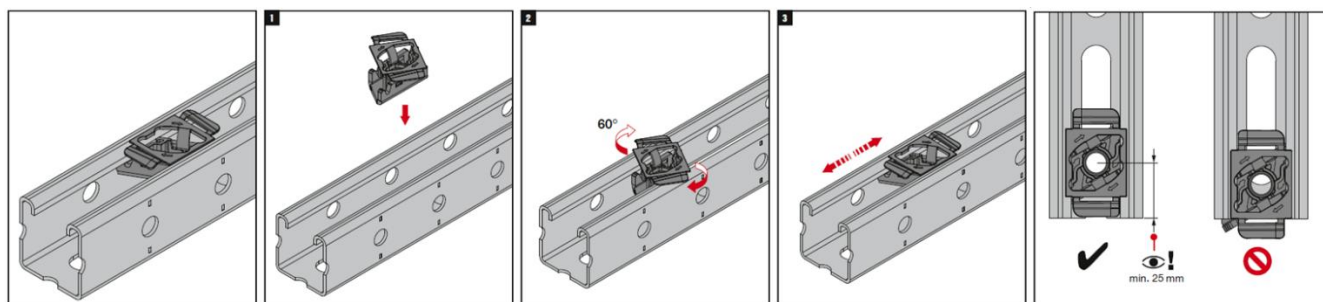
Figure B1: Installation instructions for Hilti channel connectors MT-TL M10 and MT-TL M10 OC
