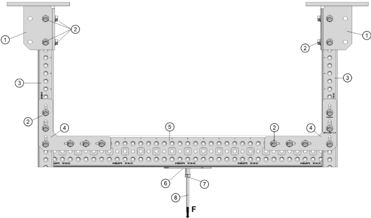
Figure B5: Hilti frame trapeze of MT System with load introduction components, closed profiles
