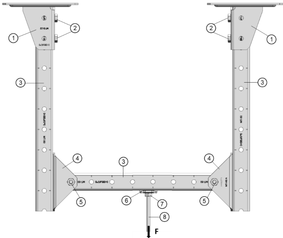
Figure B4: Hilti frame trapeze of MT System with load introduction components, MT-50 and MT-50 channels
