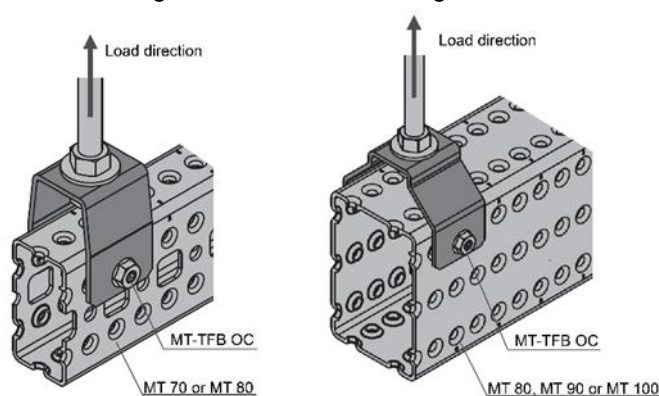
Figure B2: Assembly of Hilti MT-CTR saddle nut with Hilti MT channel
