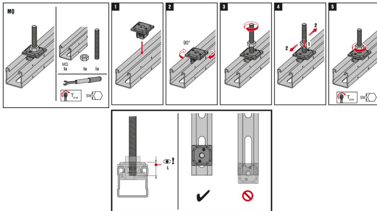
Figure B1: Installation instructions of the MQA-B saddle nut in conjunction with channel, hex-nut and threaded rod.
