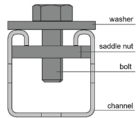
Figure B4:Assembly of Hilti MT-FP saddle nuts
