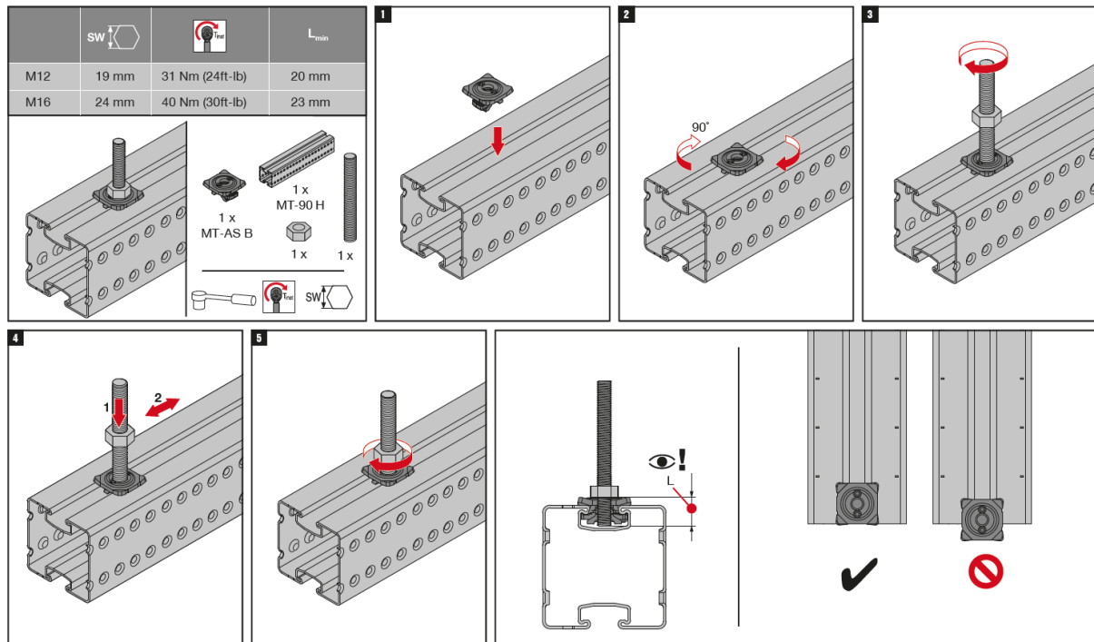
Figure B6: Instructions for use of MT-AS B M12 OC and MT-AS B M16 OC saddle nuts
