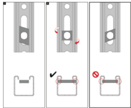
Figure B5:Installation and positioning of MT-FP saddle nuts
