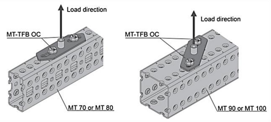
Figure B3:Assembly of Hilti MT-PCC-G saddle nut with Hilti MT channel
