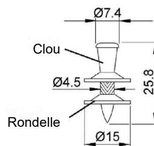
Clou X-ENP-21 HVB
