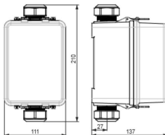
DFU 911SE dimensioned drawing and drilling plan
