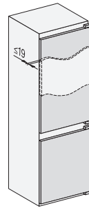
KFN7714F, KFNS7716FC, KD7714E, KD7724E, KDN7714E, KDN7724E Active, built-in (footnote*) (installation drawings)
