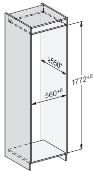
KFN7714F, KFNS7716FC, KD7714E, KD7724E, KDN7714E, KDN7724E Active, built-in (footnote*) (installation drawings)
