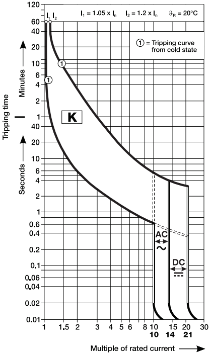
K characteristic
