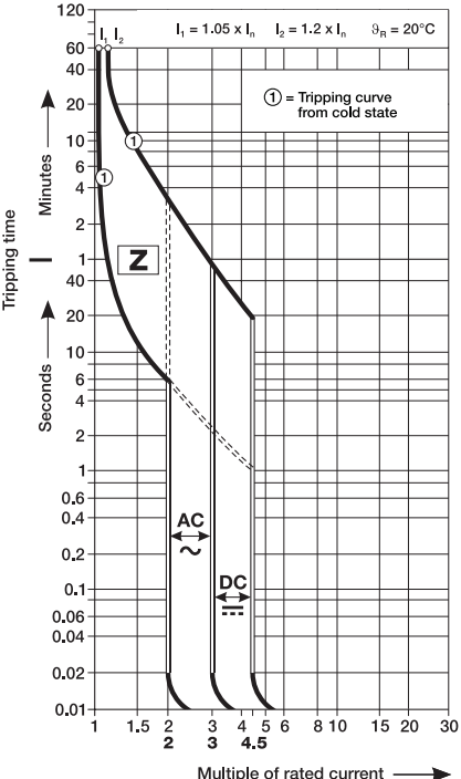
Z characteristic
