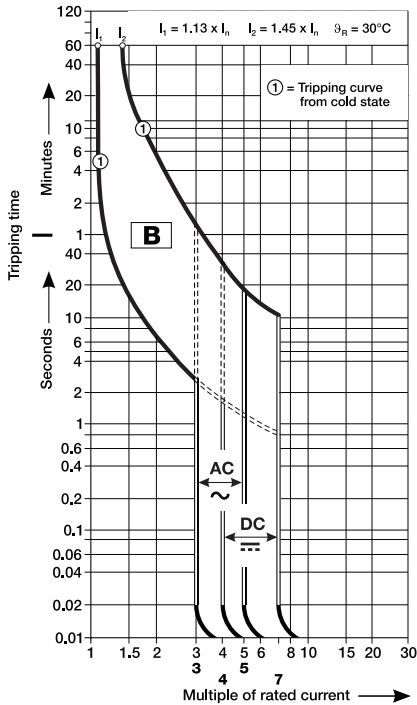
B characteristic
